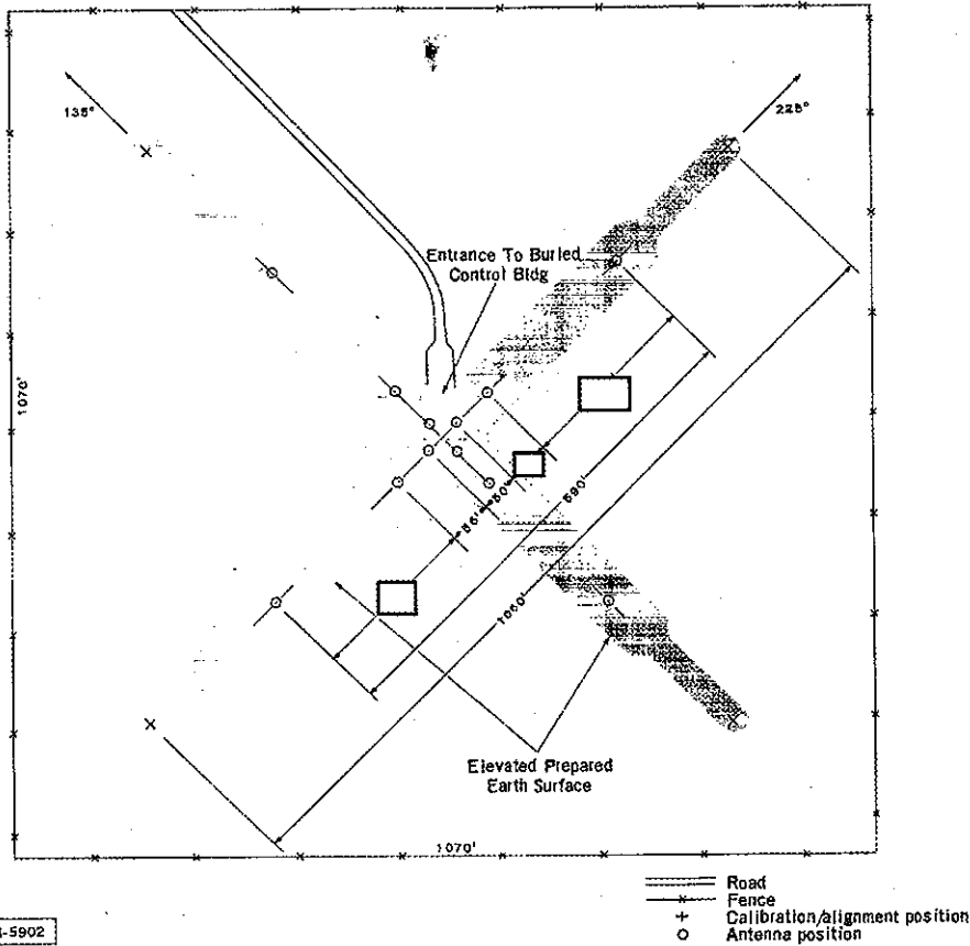
FIGURE 4. INTERFEROMETER TRACKING AREA.
